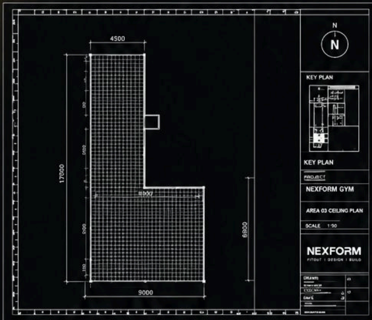
AREA 03 / CEILING PLAN
